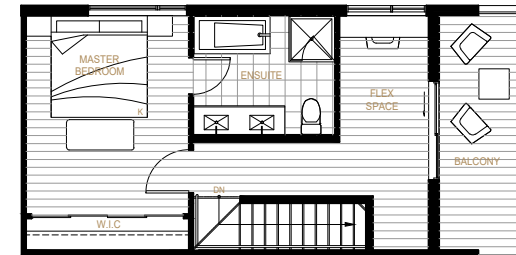
MAIN LEVEL
