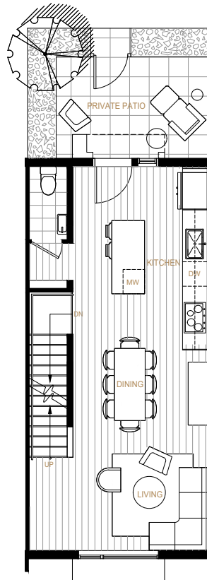
MAIN LEVEL
