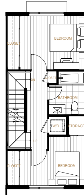
SECOND LEVEL
